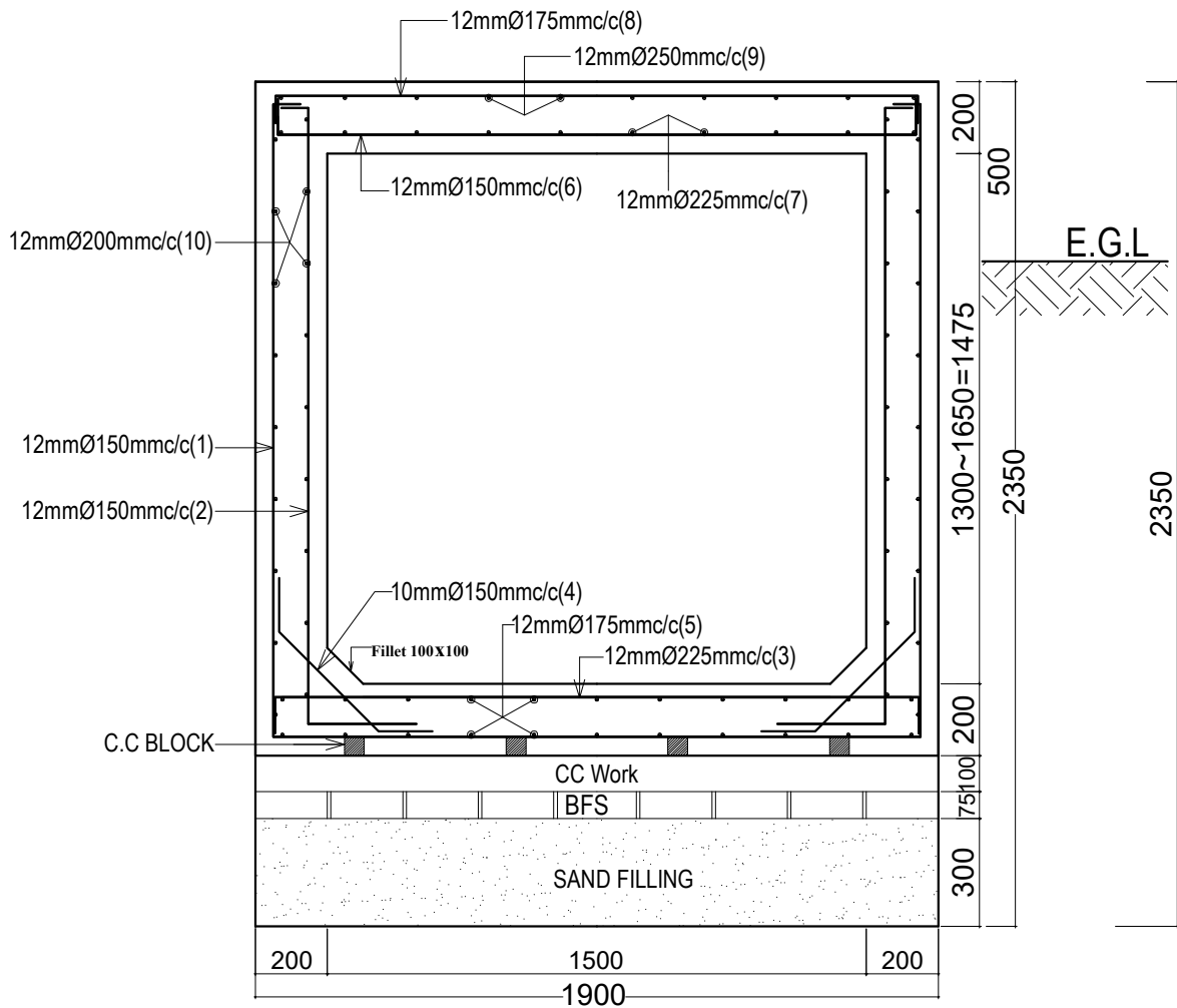
Cross Section of Drain L= 740m
